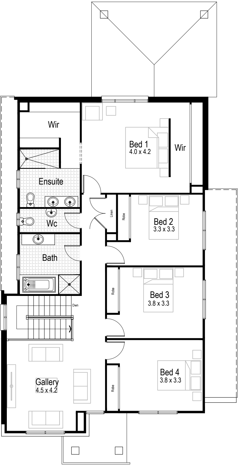
First Floor
